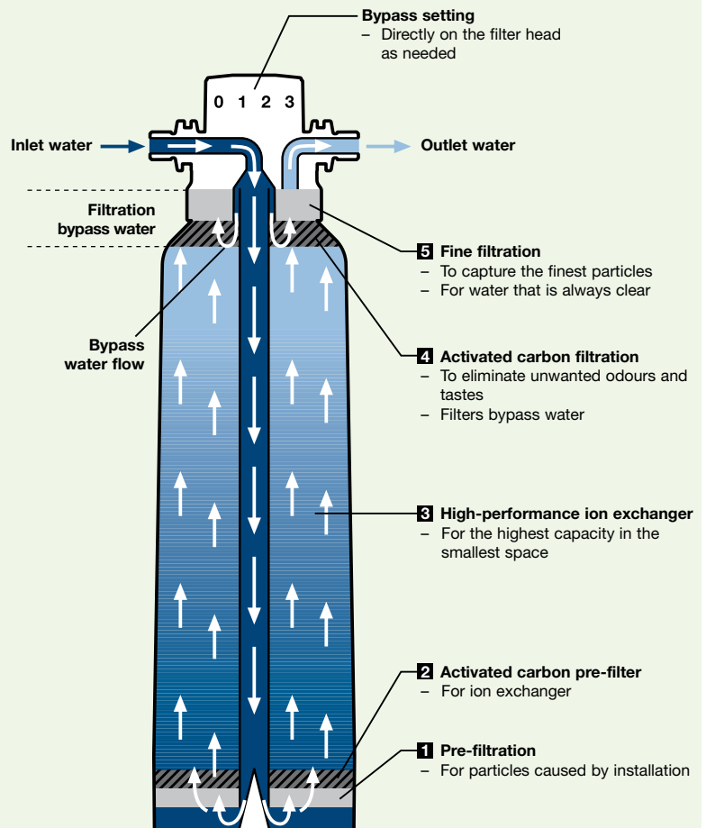
Configuration of a BWT bestclear filter cartridge with 5-way filtration
